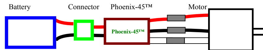
Fig 1: Motor wiring diagram
